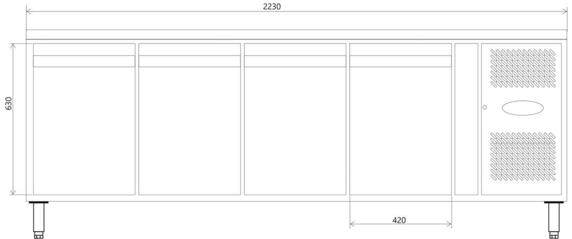
Front SK6410+SP
